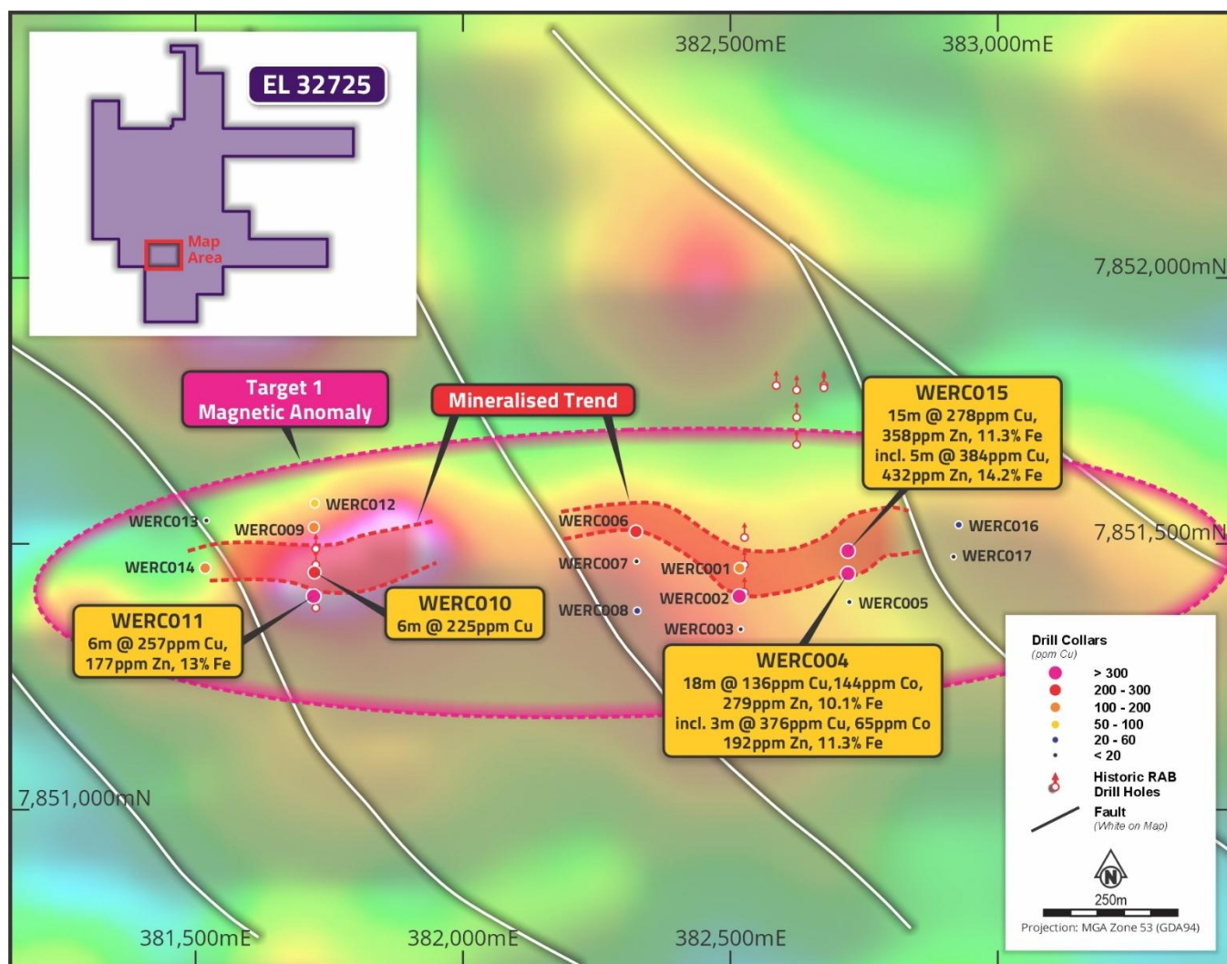
Figure 2: Warrego East EL32725, Target 1 magnetic anomaly with recent drilling interpreted mineralisation and structures
