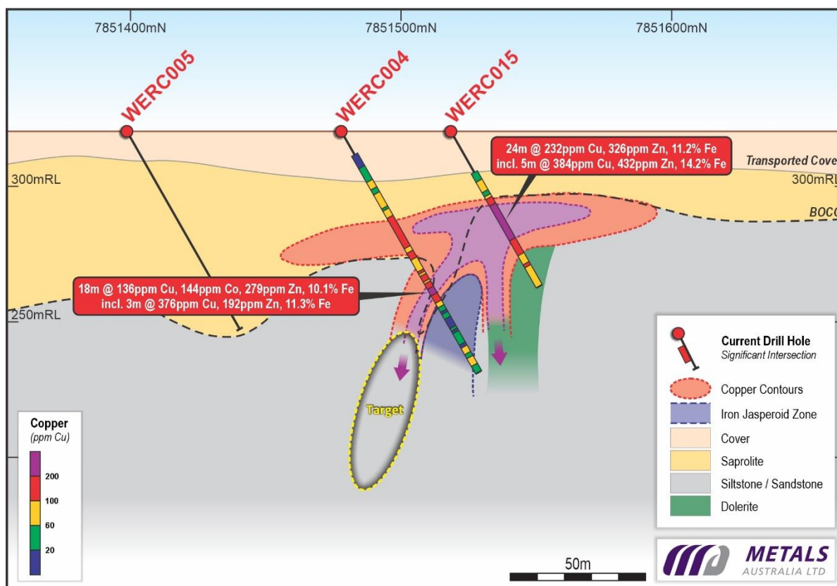
Figure 4: Warrego East, Target 1 cross section 382,530mE showing recent and previous drilling results and targets
