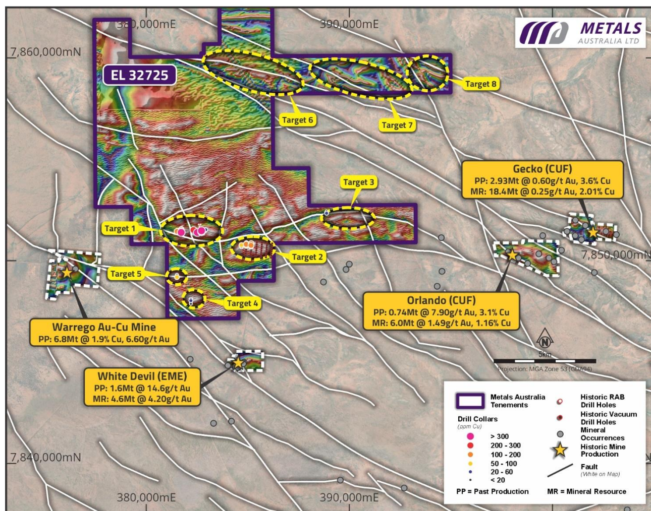
Figure 1: Warrego East EL32725 Total Magnetic Intensity (TMI) with major Cu-Au deposits, MLS targets and drilling
