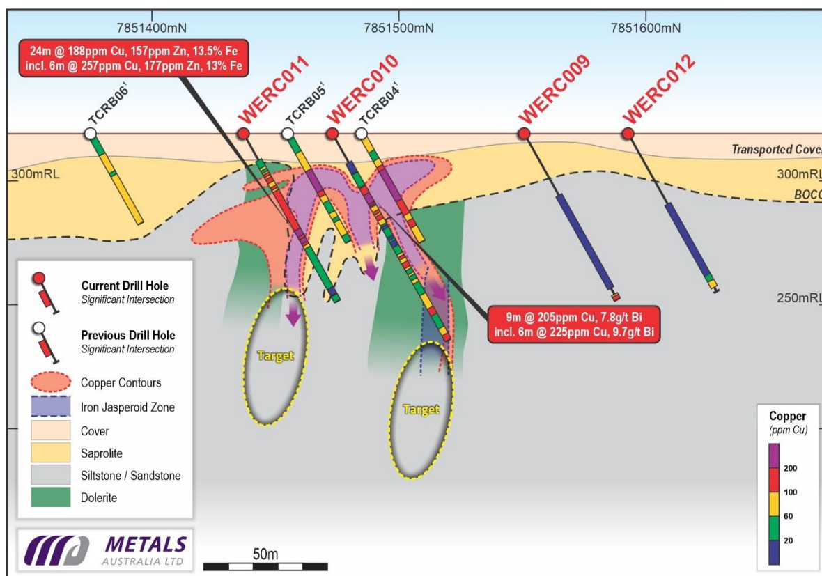
Figure 3: Warrego East, Target 1 cross section 381,730mE showing recent and previous drilling results and targets
